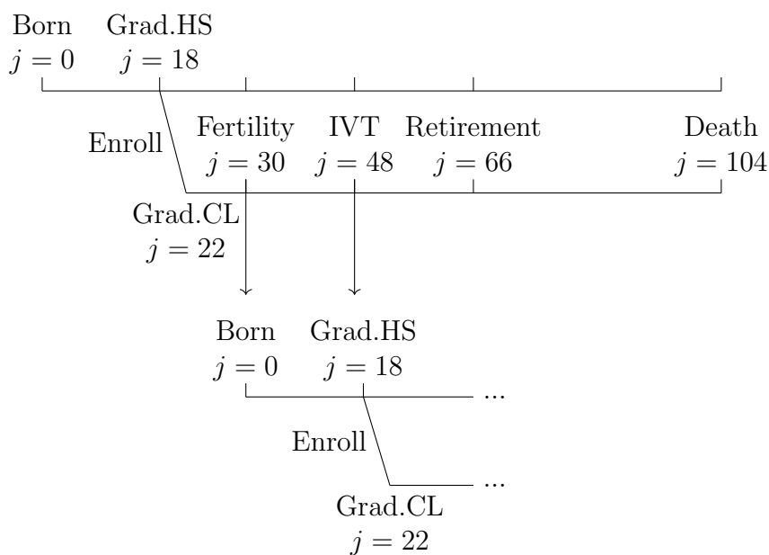
Fig 1: Model's lifecycle.
